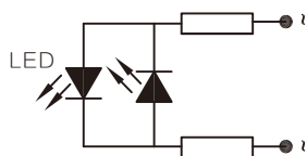
适用交流: 6.3VAC, 12VAC, 24VAC, 48VAC, 110VAC, 220VAC For 6.3VAC, 12VAC, 24VAC, 48VAC, 110VAC, 220VAC
