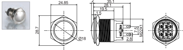
弧面按钮
